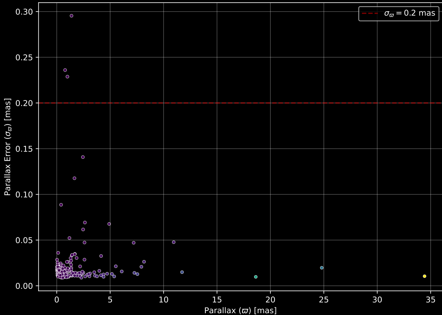
APOGEE DR17 Field: [M13] Parallax Quality (n= 333)
