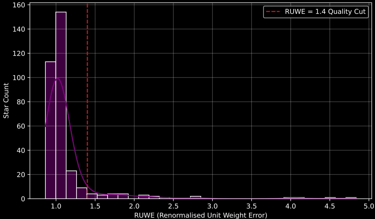
GAPOGEE DR17 Field [M13] RUWE Distribution (n= 326)
