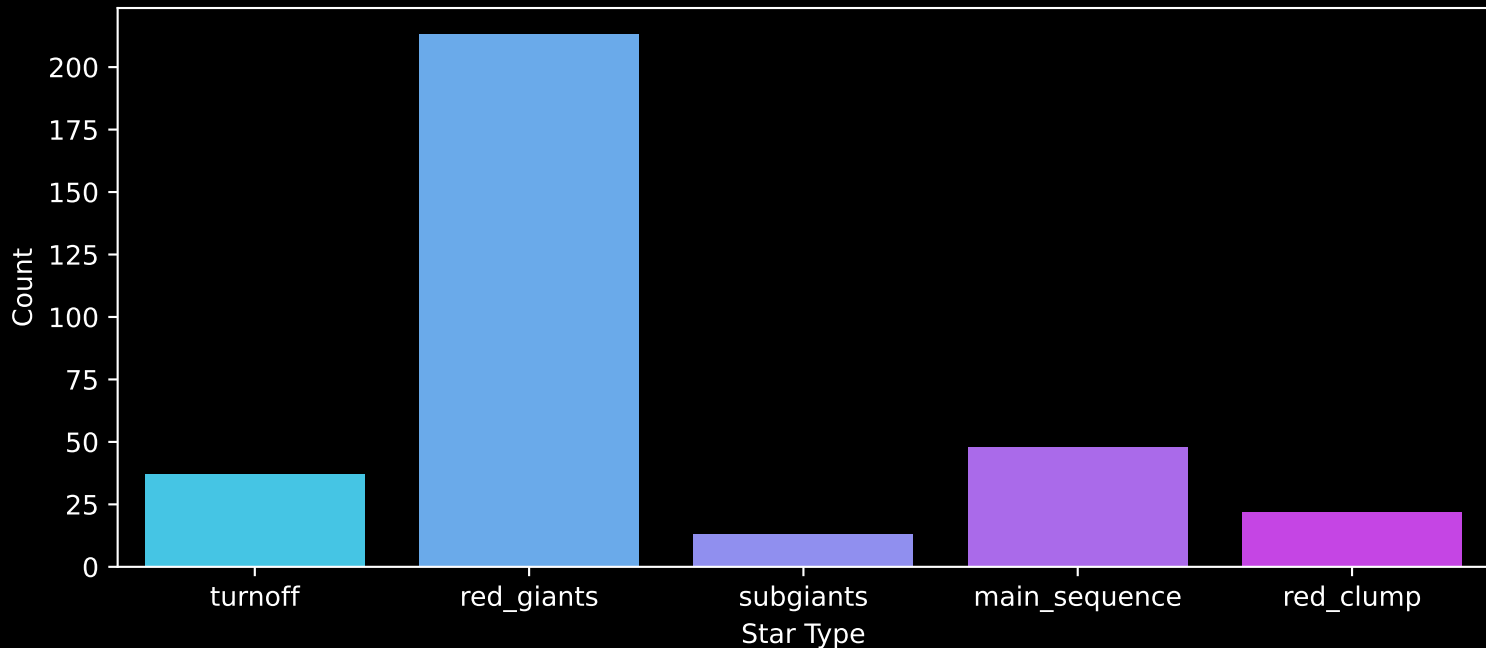
APOGEE DR17 Field: [M13] Count plot of Star Type
