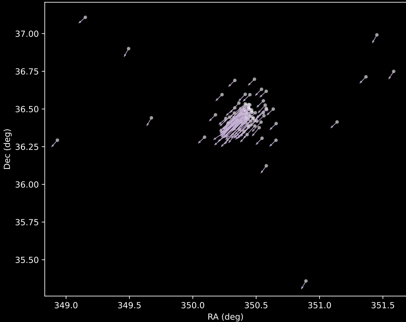
APOGEE DR17 Cluster 9 Proper Motion Vectors (n=92)
