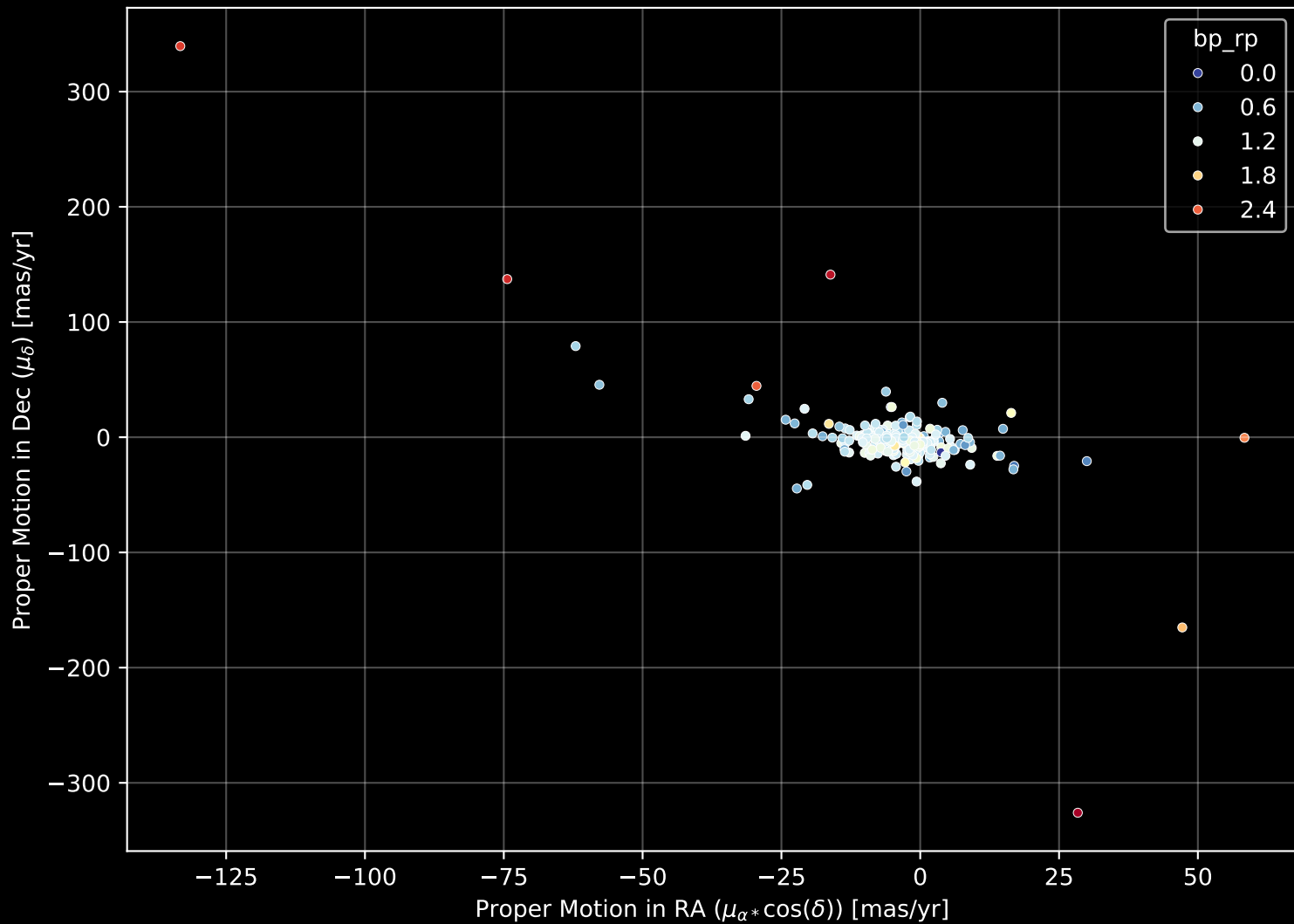
APOGEE DR17 Field: [M13] Proper Motion Diagram (n= 333)
