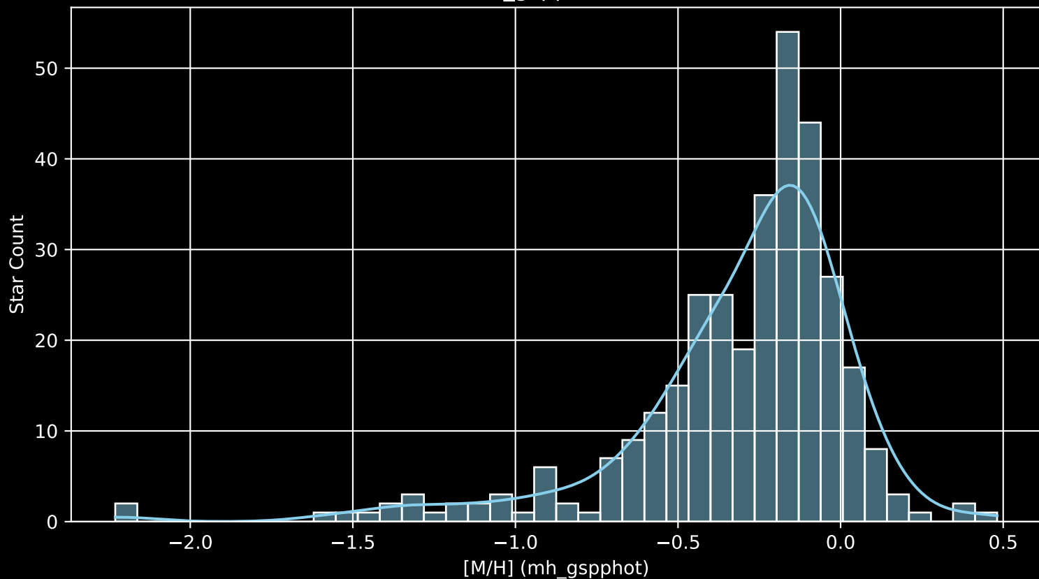
APOGEE DR17 Field: [M13 [M/H] (mh_gspphot) (n= 333)
